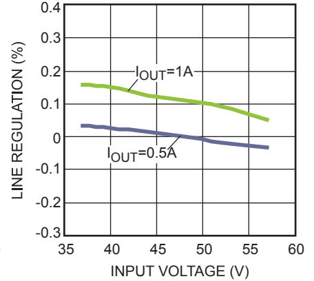
Line Regulation
