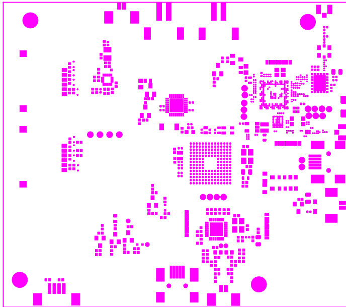
09-Solder Mask Top
