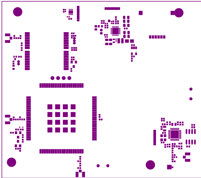
10-Solder Mask Bottom
