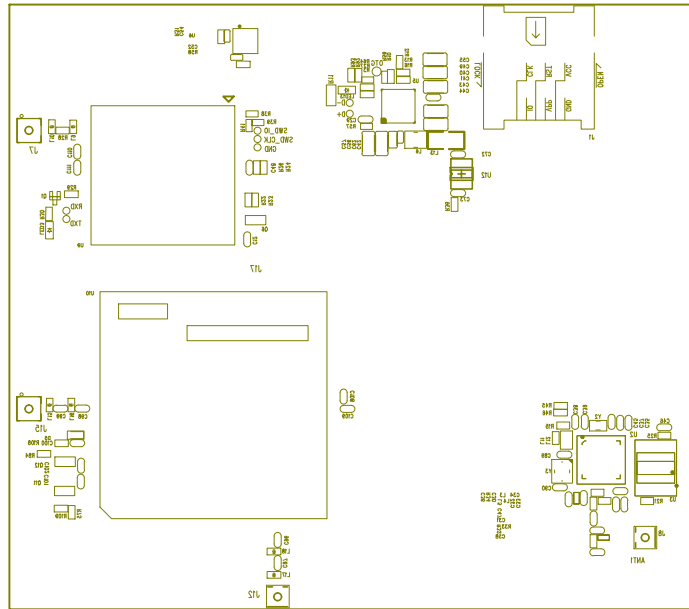
06-Silkscreen Bottom
