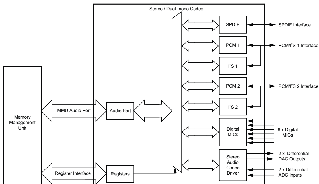
Figure 10.1: Audio Interface
