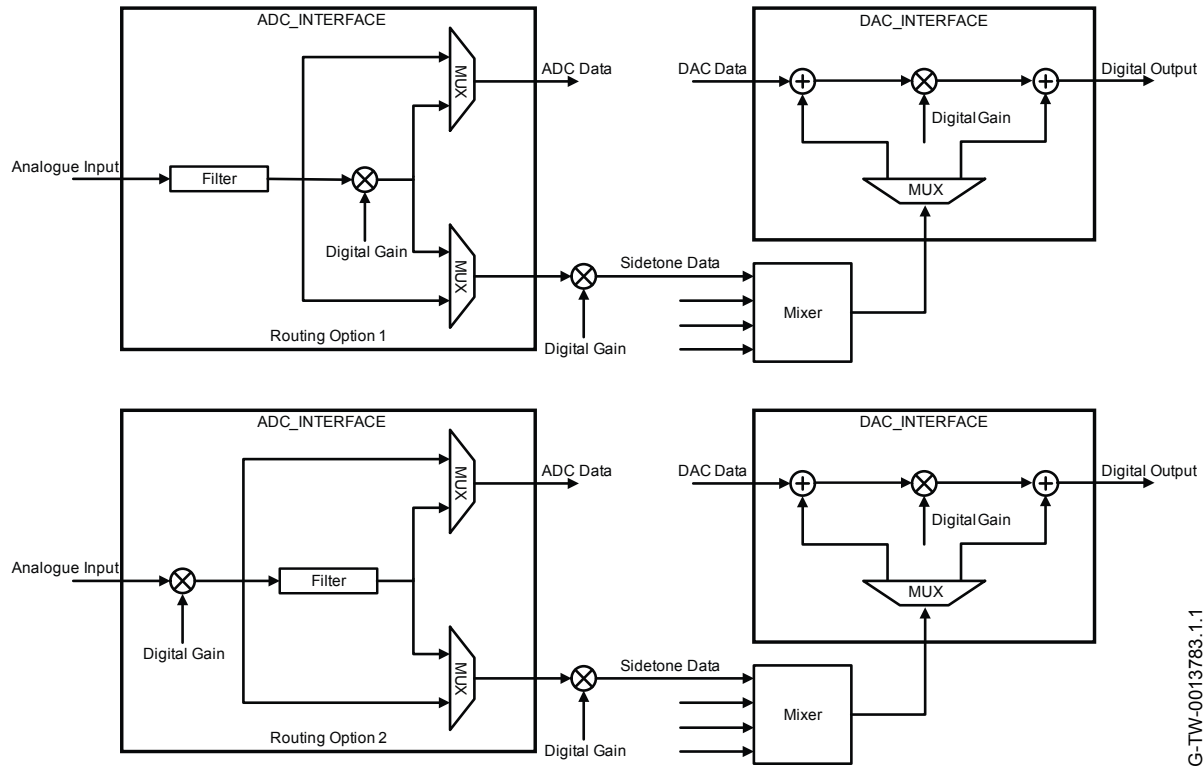
Figure 10.10: Side Tone
