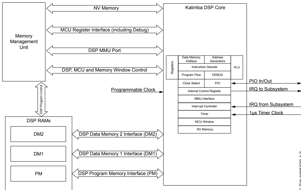
Figure 6.1: Kalimba DSP Interface to Internal Functions
