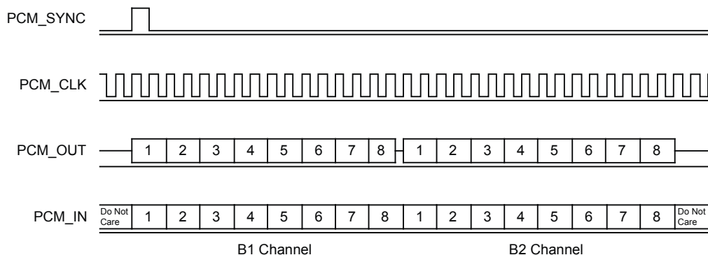
Figure 10.16: GCI Interface
