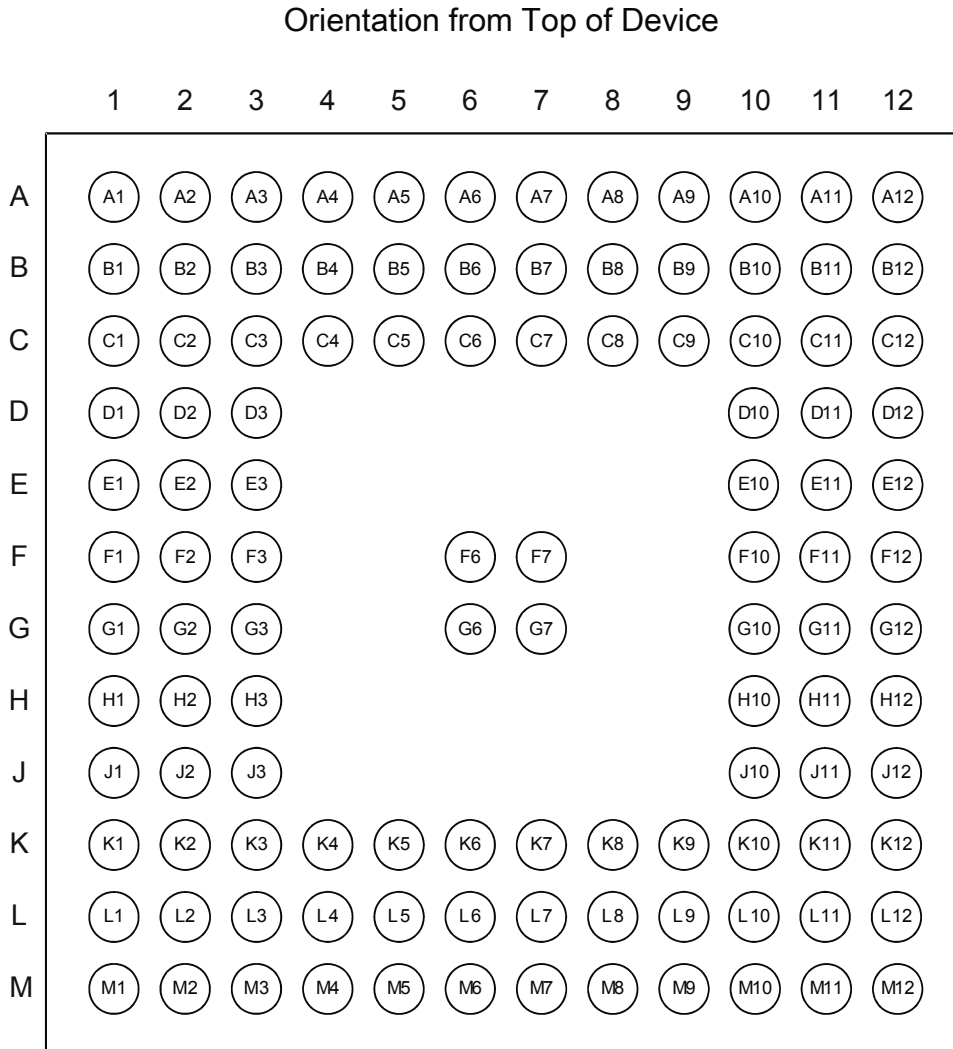
Figure 1.1: Pinout Diagram
