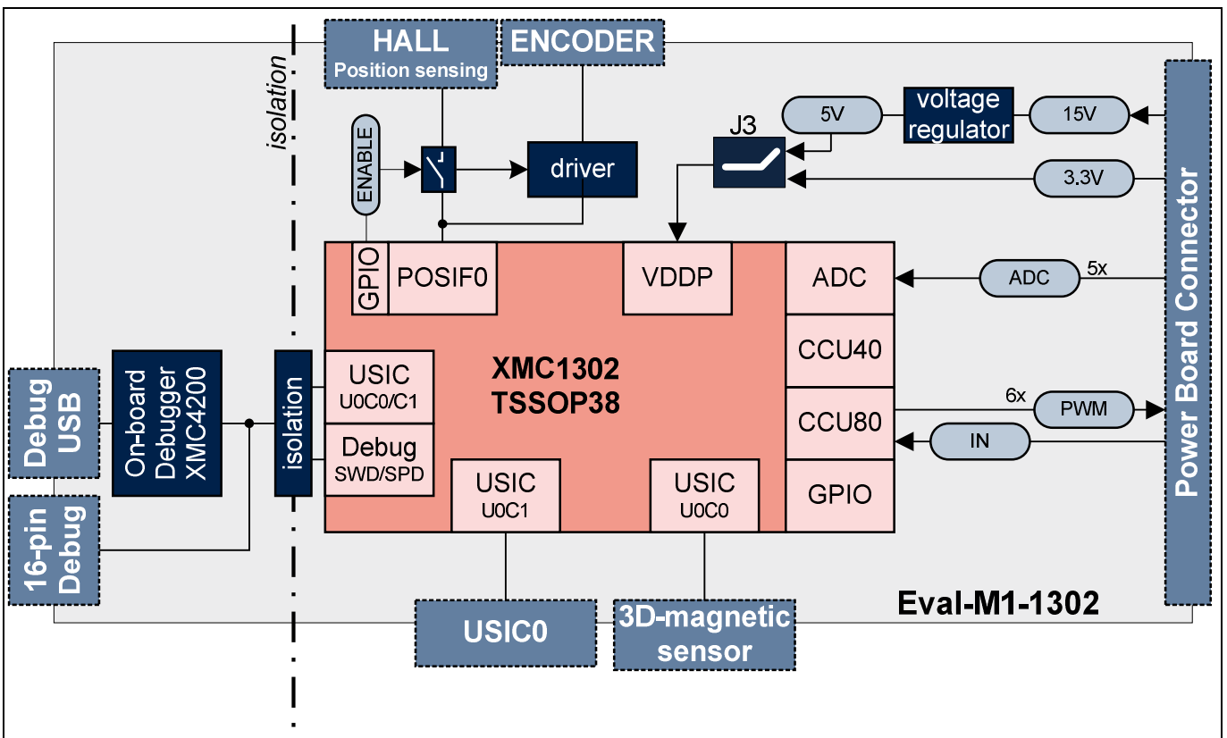
Figure 1 Block Diagram of the Eval-M1-1302
