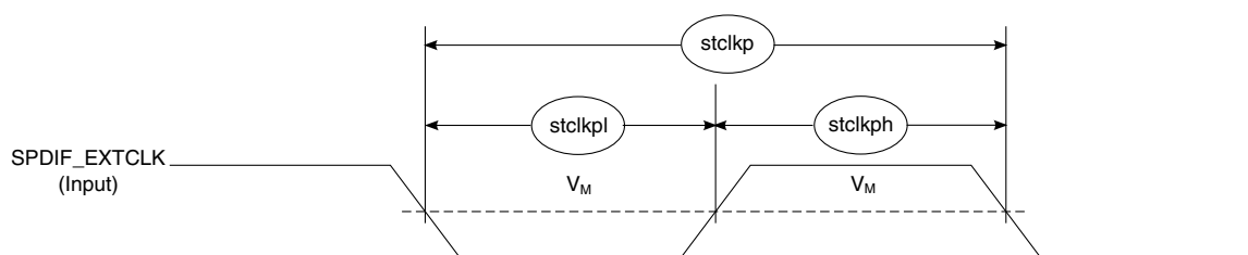
Figure 51. SPDIF_EXTCLK timing
