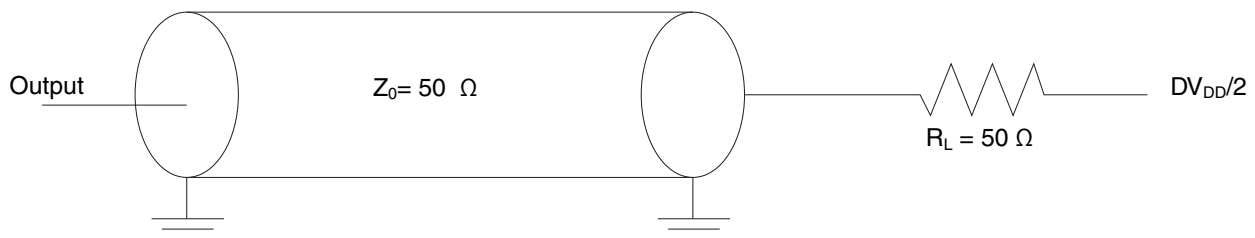
Figure 70. I 2 C AC test load
