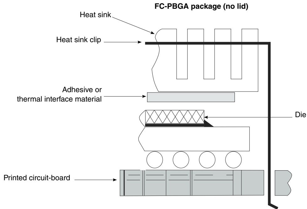
Figure 92. Package exploded, cross-sectional view-FC-PBGA (no lid)
