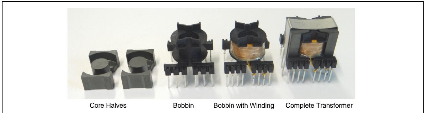
Figure 3.3 PQ16/20 Transformer
