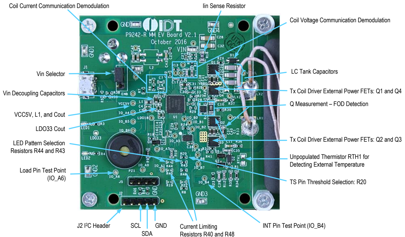
Figure 8. P9242-R3 V2.1 Evaluation Board Details
