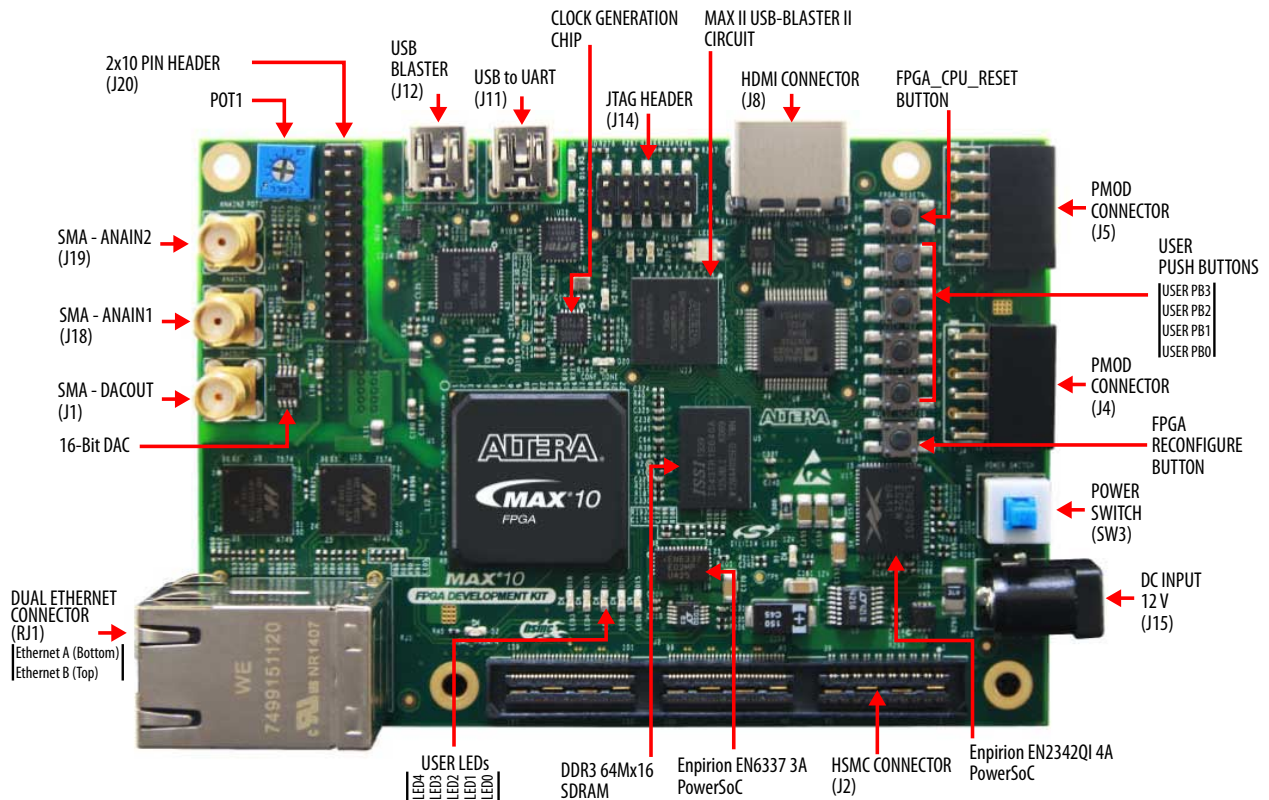
Figure 1-1: MAX 10 FPGA Board Components (Top)
