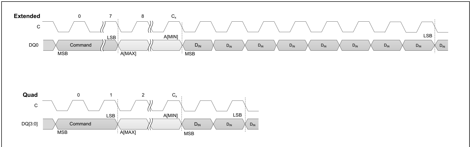
Figure 34. Memory-Write Timing
