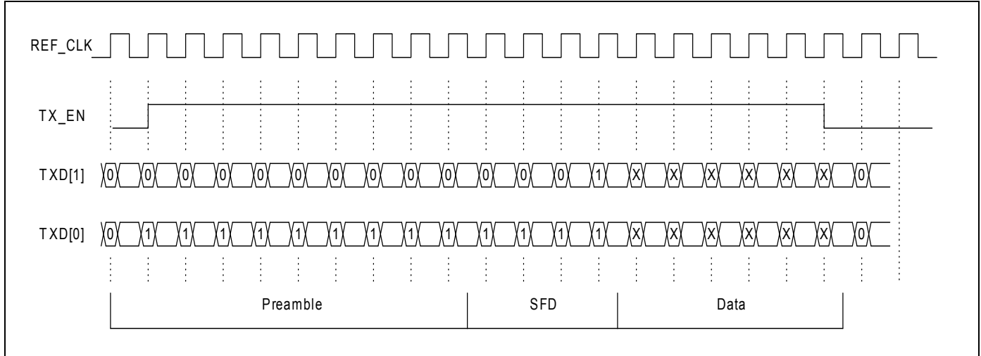
Figure 20. RMIIT Transmit Packet Timing
