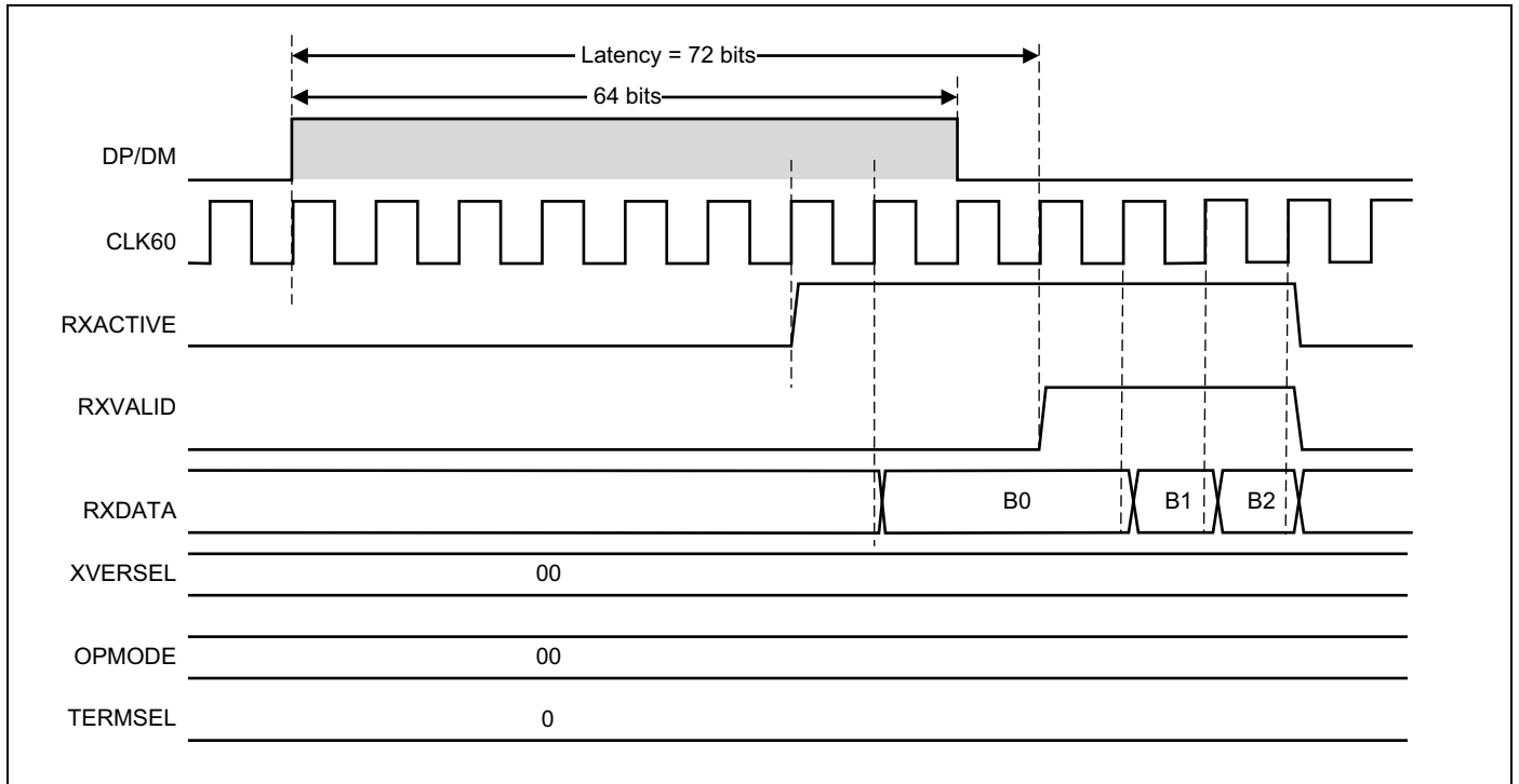
Figure 38. USB 2.0 High-Speed Mode Receive Timing
